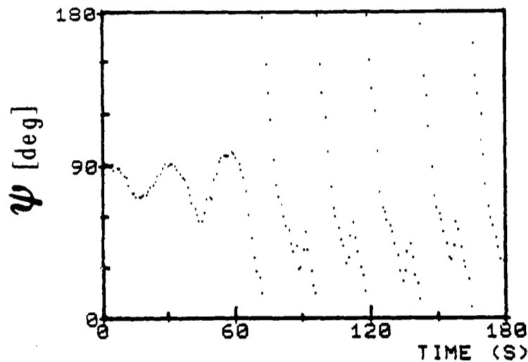
FIGURE 4. Plot of the angle \psi of the probe beam vs. time. The pump power is P=111 mW and ellipticity s_3(0)=.81
